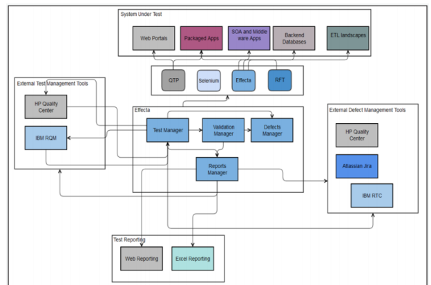
Figure 1. A look at the architecture of the Effecta accelerator
